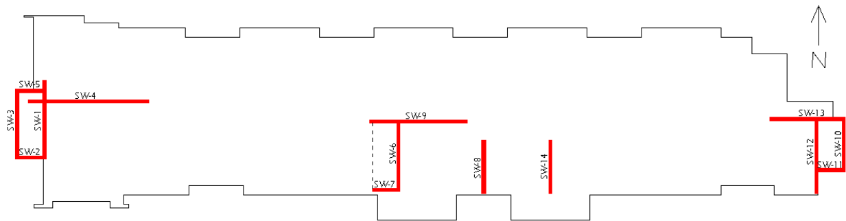
(FIGURE 52) Shear Wall Layout
