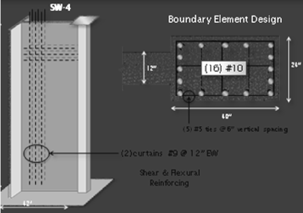
(FIGURE 57) Shear Wall 4 Re-Design Illustration
